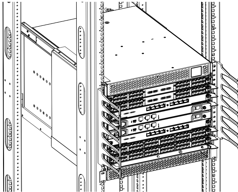
FIGURE 5 Vertical cable management finger assemblies
