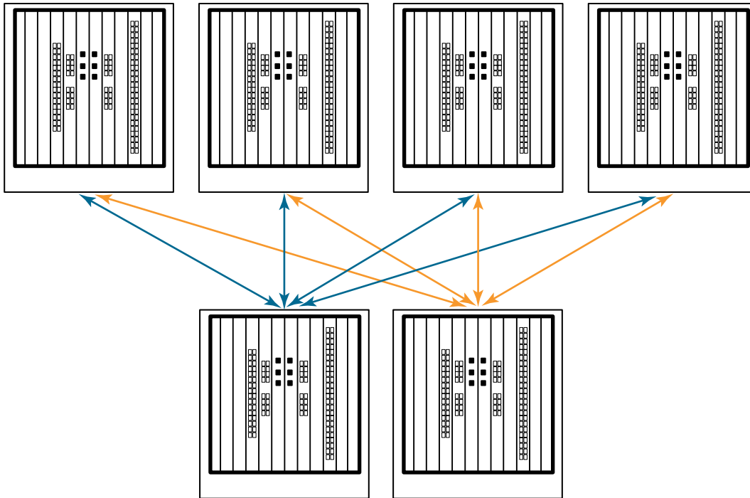
FIGURE 9 Topologie core/edge ICL DCX 8510
